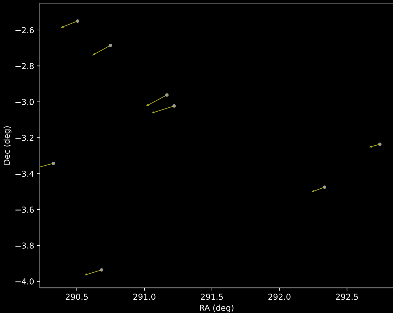
APOGEE DR17 Cluster 16 Proper Motion Vectors (n=8)
