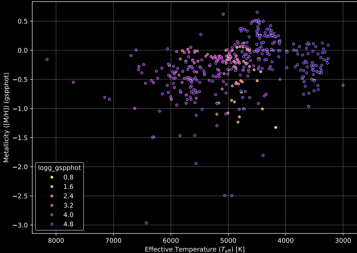
APOGEE DR17 Field: [300+60] Stellar Population Parameters (n= 414)
