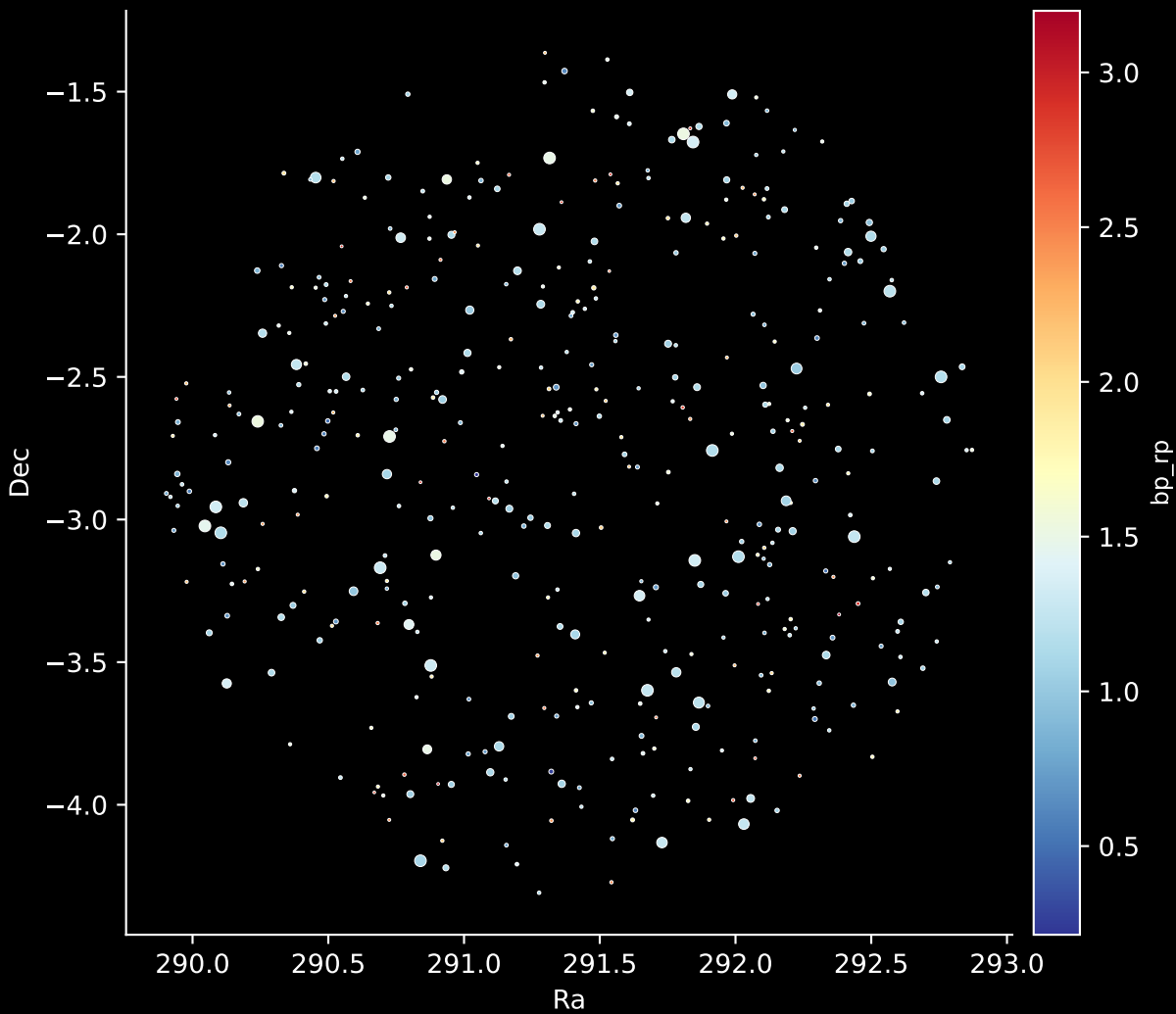
APOGEE DR17 Field: [300+60] Stars: 414
