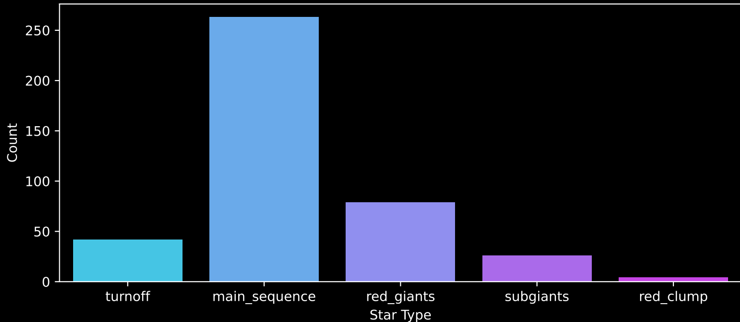
APOGEE DR17 Field: [300+60] Count plot of Star Type
