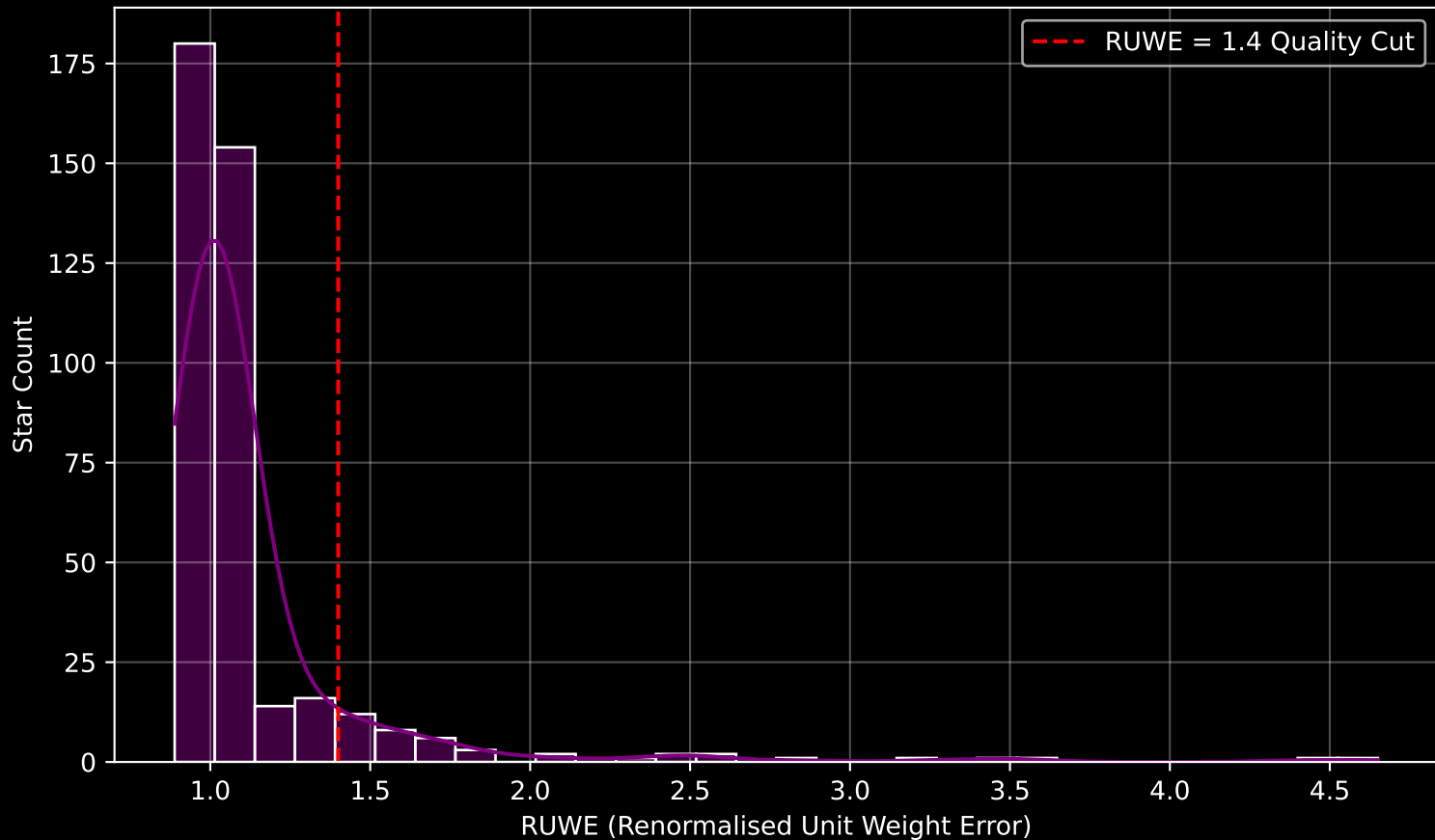
GAPOGEE DR17 Field [300+60] RUWE Distribution (n= 406)
