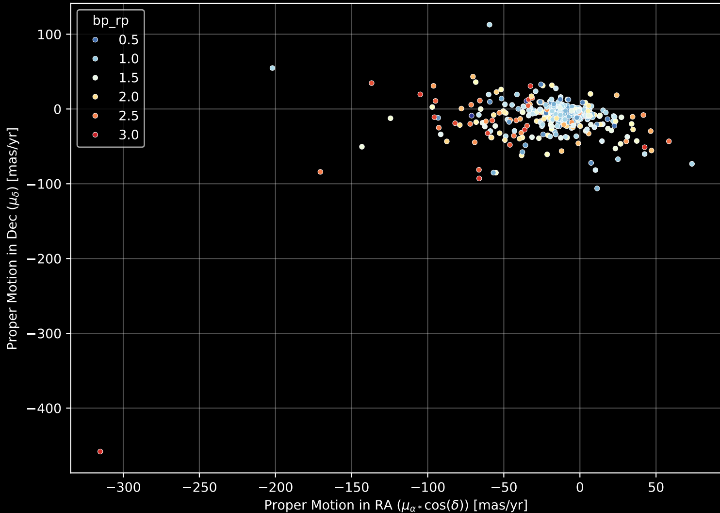
APOGEE DR17 Field: [300+60] Proper Motion Diagram (n= 414)
