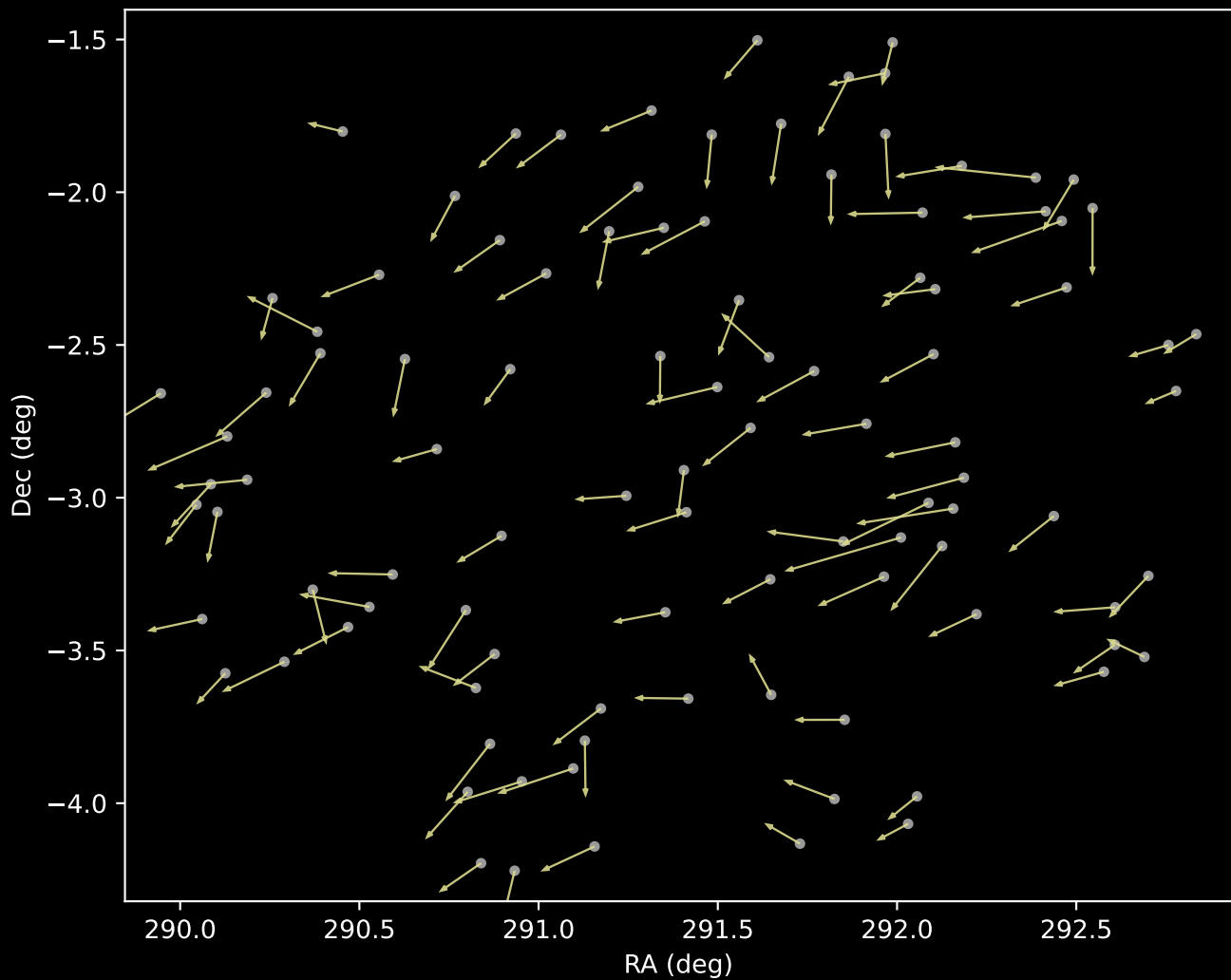
APOGEE DR17 Cluster 17 Proper Motion Vectors (n=101)
