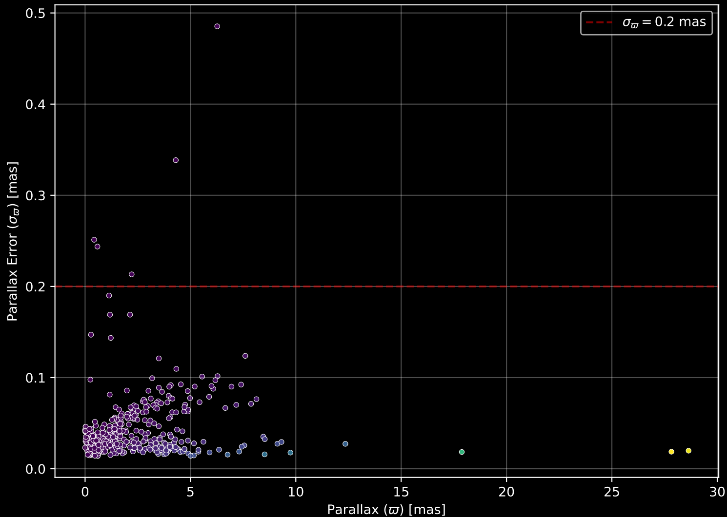
APOGEE DR17 Field: [300+60] Parallax Quality (n= 414)
