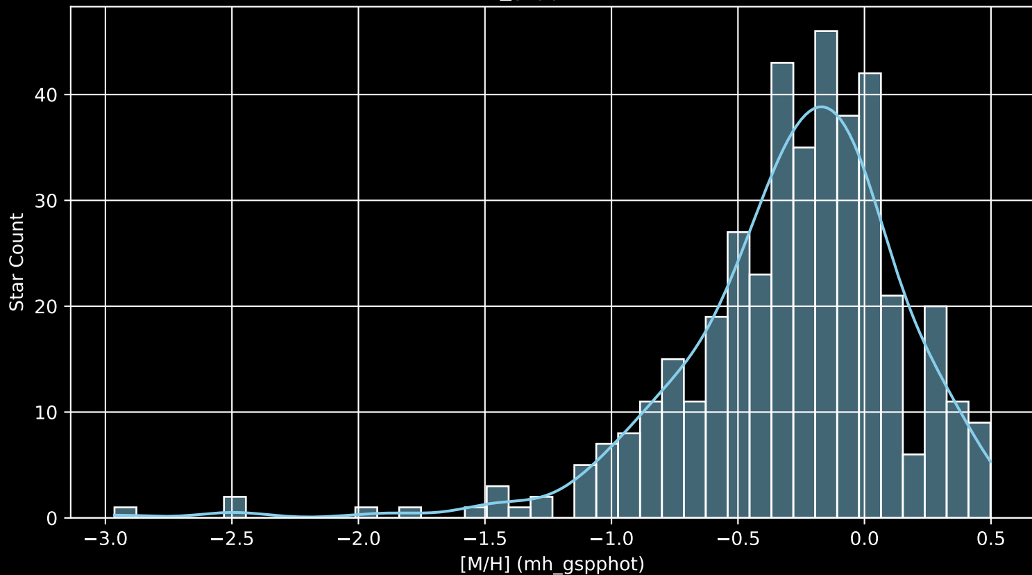
APOGEE DR17 Field: [300+60 [M/H] (mh_gspphot) (n= 409)
